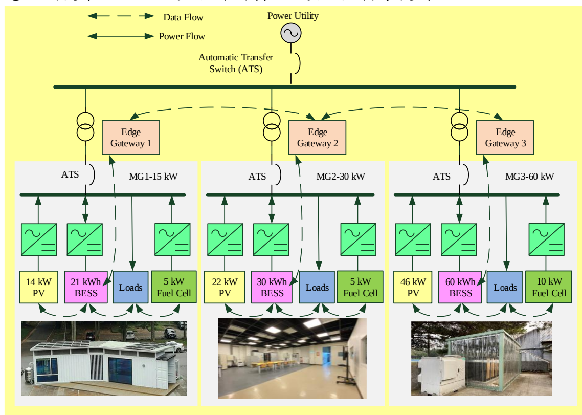
Field Implementation of 100-kW Smart Multi-Level Microgrid in NCU
